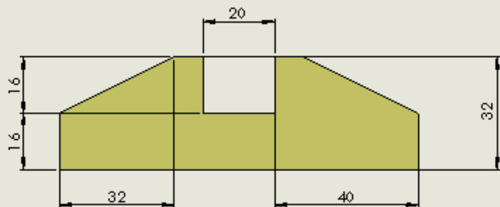
Plan
